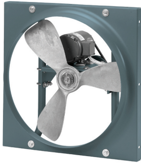
Axial Wall Fan AMCA Certified for Air
